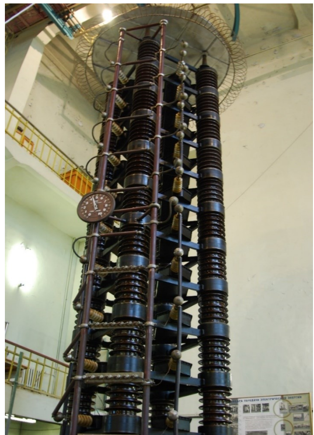
Fig. 2 – The pulse voltage generator of 2.4 MV.
