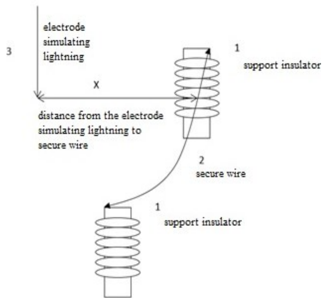
Fig. 1 – General view of the model. 1 support insulator, 2 secure wire, 3 electrode simulating lightning, X distance from the electrode simulating lightning to secure the wire.
