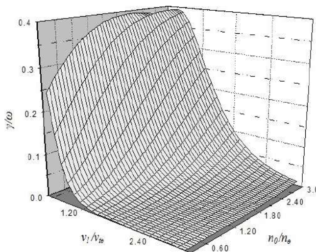
Fig. 3 – Dependence of EMR damping on the non-equilibrium parameter of solid-state plasma
